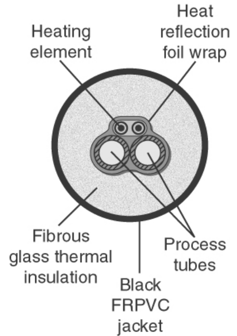
2262 Dual Tube
